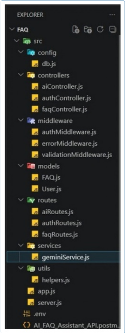
Fig. 1 - Actual project folder structure (VS Code Explorer): FAQ/src/{config, controllers, middleware, models, routes, services, utils}, app.js, server.js, .env, and the team's Postman collection Full source is version-controlled and available at https://github.com/sabarivasan-2105/AI_FAQ_Assistant_API . The backend runs on Node.js/Express with MongoDB (Mongoose) and exposes Auth, FAQ and AI route groups, with both AI-generation endpoints isolated behind services/geminiService.js .
